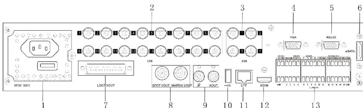
Fig. 2 1.5U case model without DVD writer
