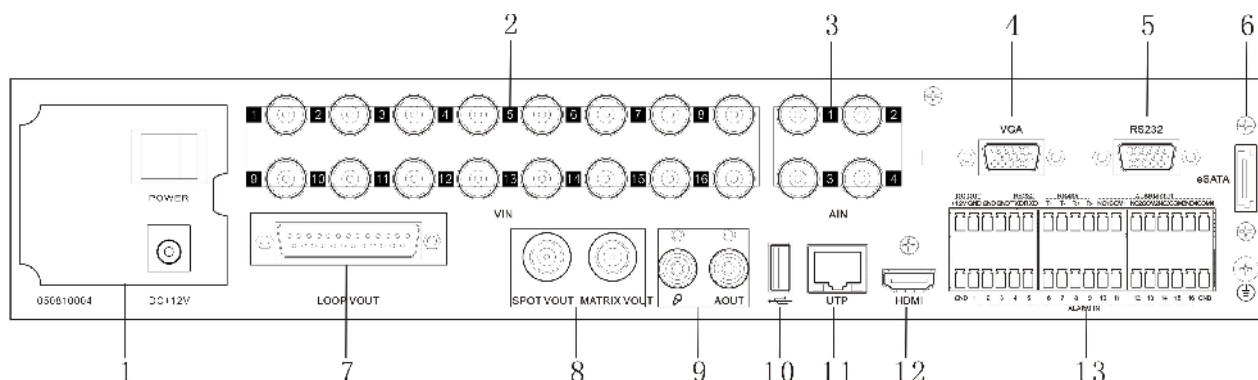
Fig.3 1.5U case model with DVD writer
